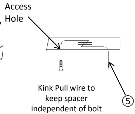
Example of pull wire procedure Figure 2
